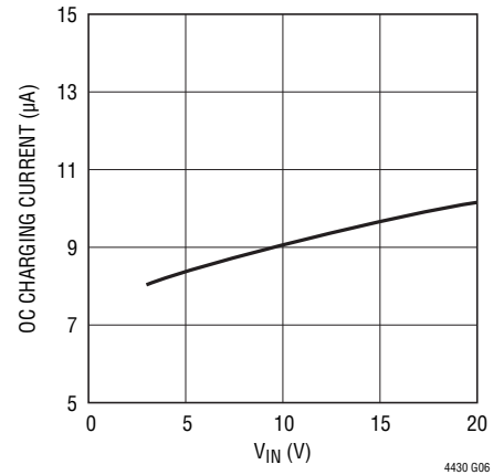
OC Charging Current vs Input Voltage
