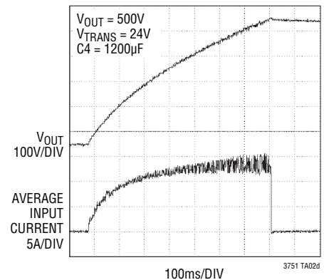
Charging Waveform
