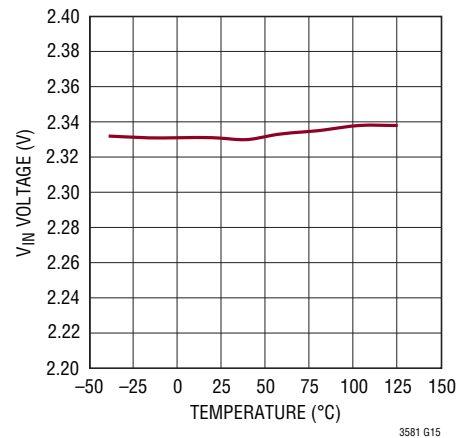
Internal UVLO
