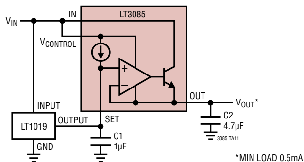
Reference Buffer
