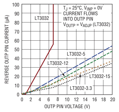
Reverse OUTP Pin Current
