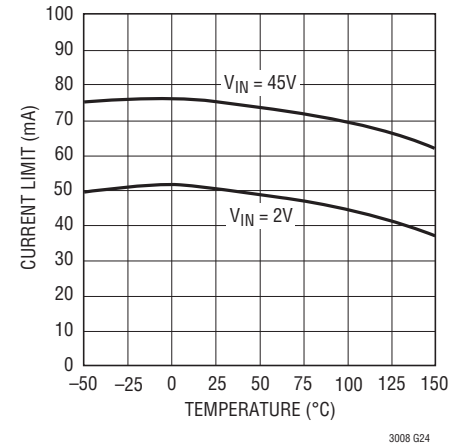
Current Limit
