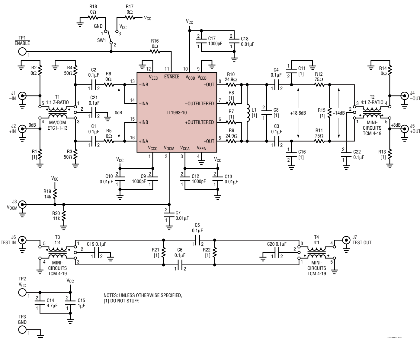
Demo Circuit DC800A Schematic (AC Test Circuit)
