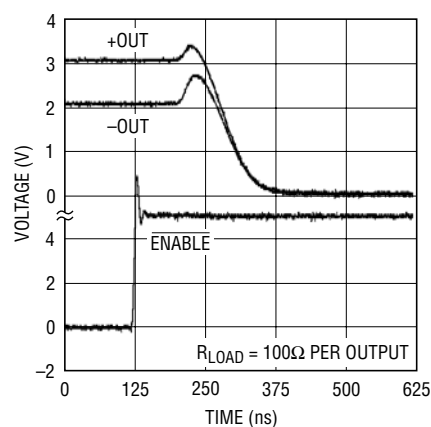
Turn-Off Time
