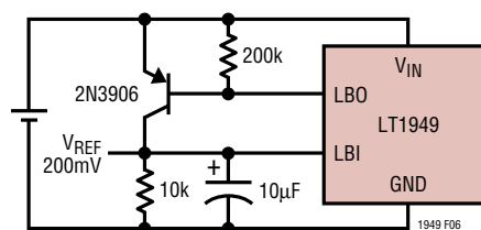
Figure 6. Accessing 200mV Reference
