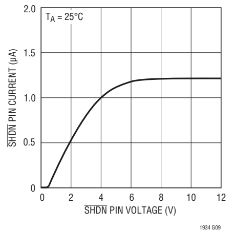
SHDN Bias Current vs SHDN Voltage
