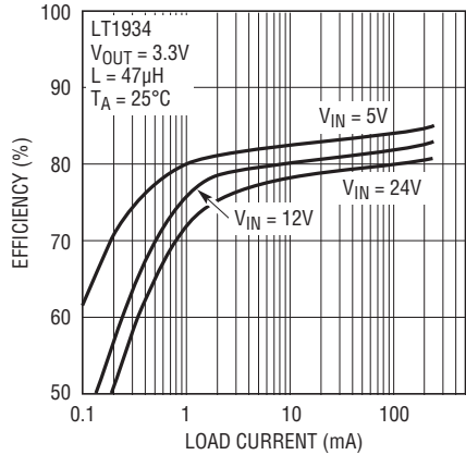
LT1934 Efficiency, V_{OUT} = 3.3V
