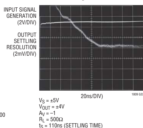
0.01% Settling Time
