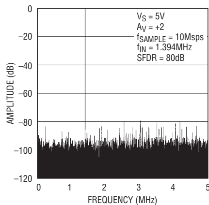
Figure 7. 4096 Point FFT Response
