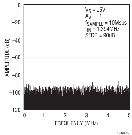
Figure 5. 4096 Point FFT Response
