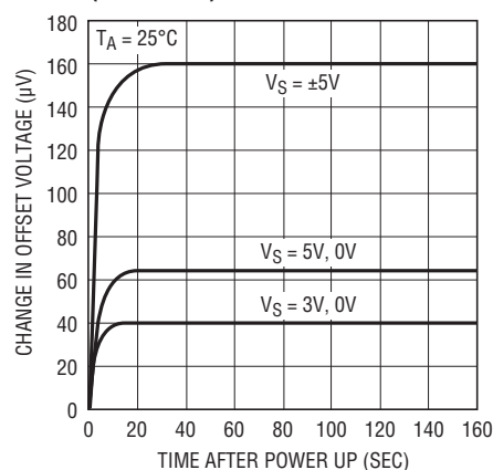
Warm-Up Drift vs Time (LT1809S8)
