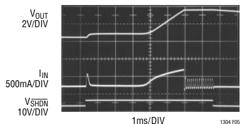
Figure 5. Start-Up Response with 1μF/1MΩ Components in Figure 2 Added. Input Current Is More Controlled. V OUT Reaches 5V in 6ms. Output Drives 20mA Load
