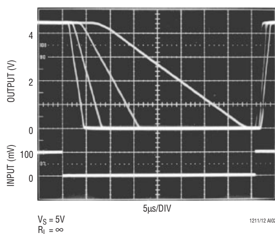
LT1211 Comparator Response (–) 20mV, 10mV, 5mV, 2mV Overdrives
