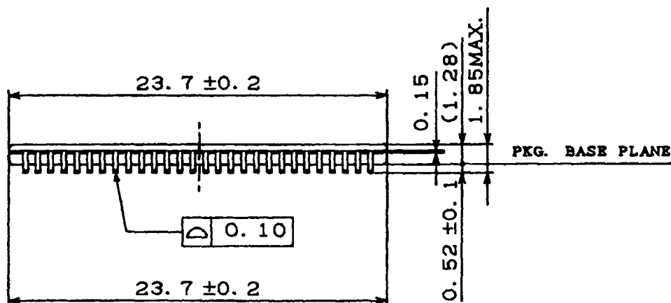
DETAIL A
