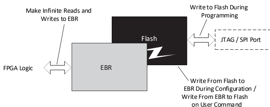
Figure 2.16. FlashBAK Technology
