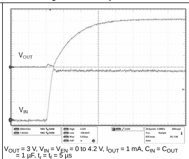
Figure 31. Startup transient
