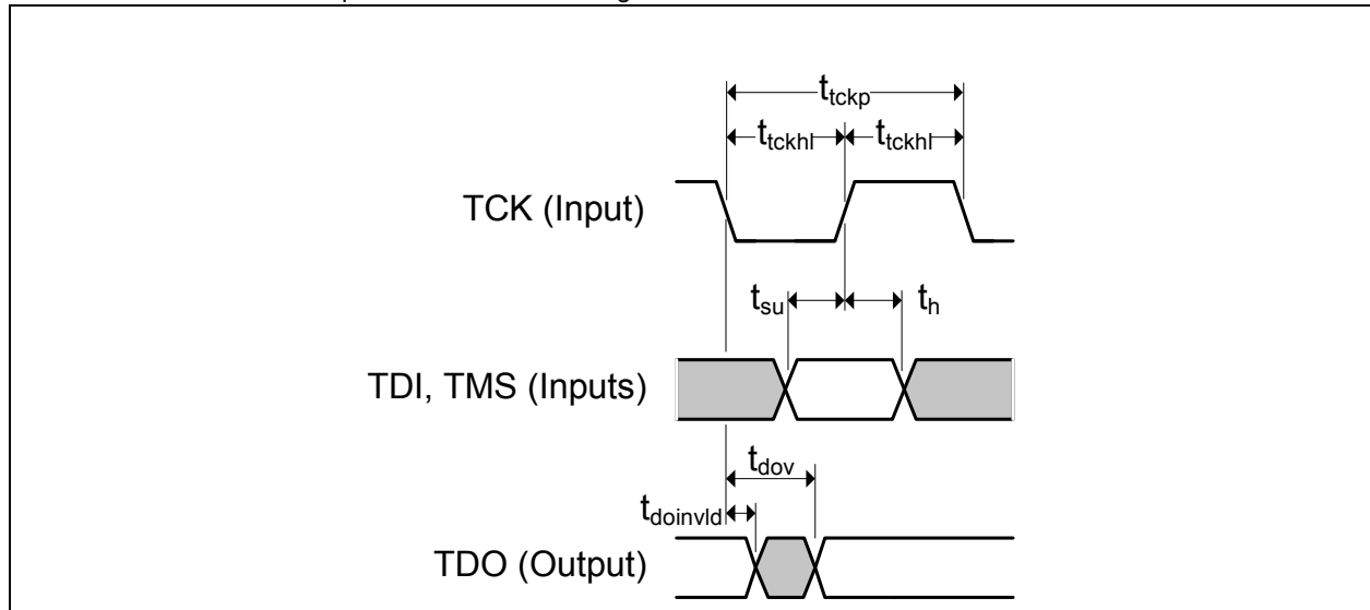
Figure 6.10 JTAG Timing
