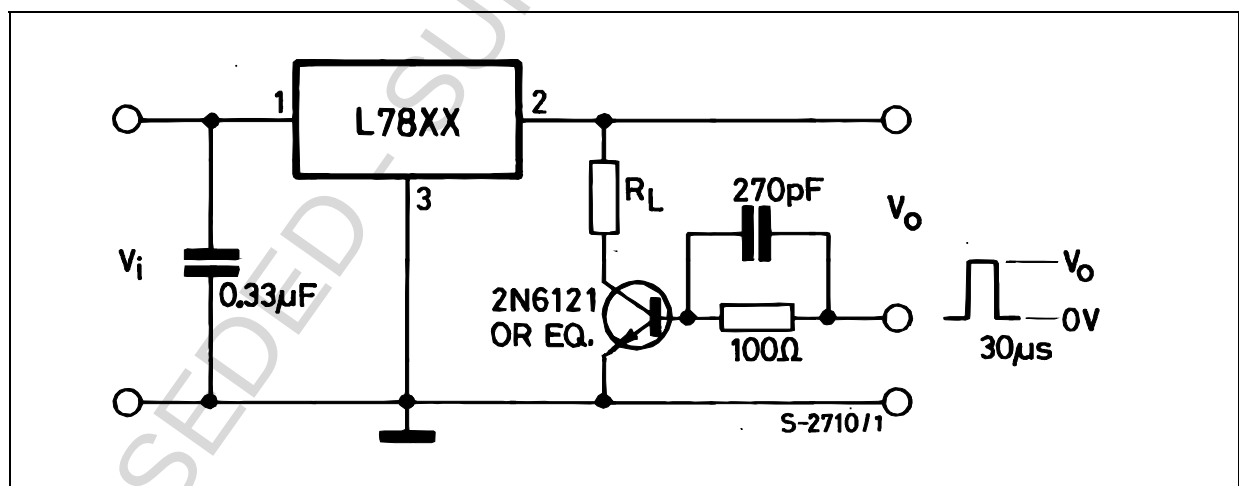
Figure 2 : Load Regulation
