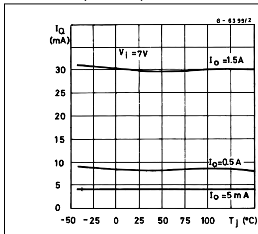
Figure 12. Quiescent current vs temperature (L4940V5)
