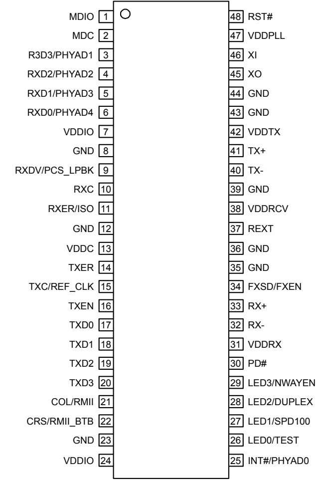
48-Pin SSOP (SM)
