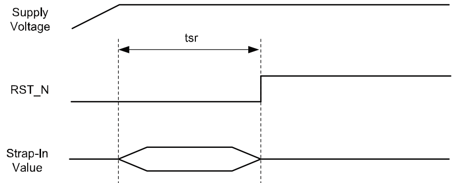
Figure 9. Reset Timing
