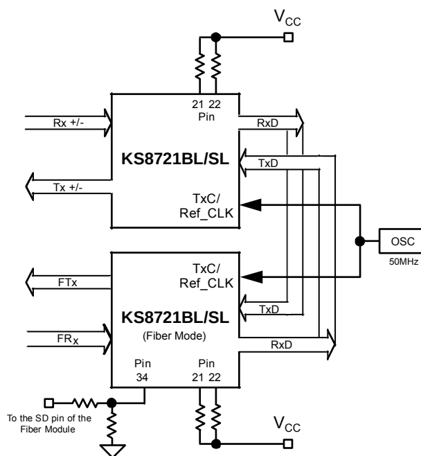
Figure 3. Fiber Module
