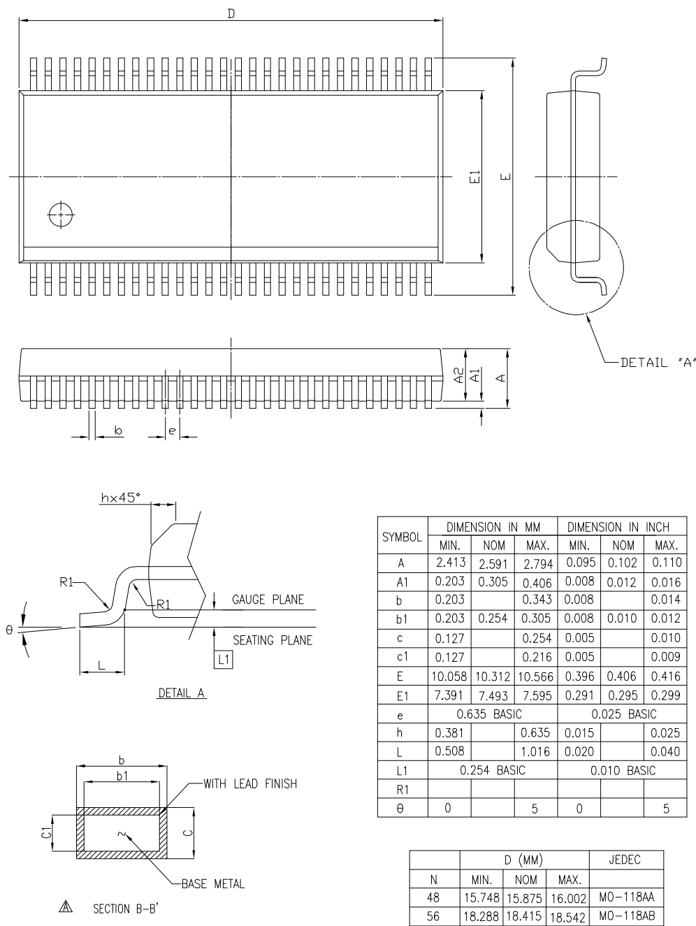
48-Pin SSOP (SM)
