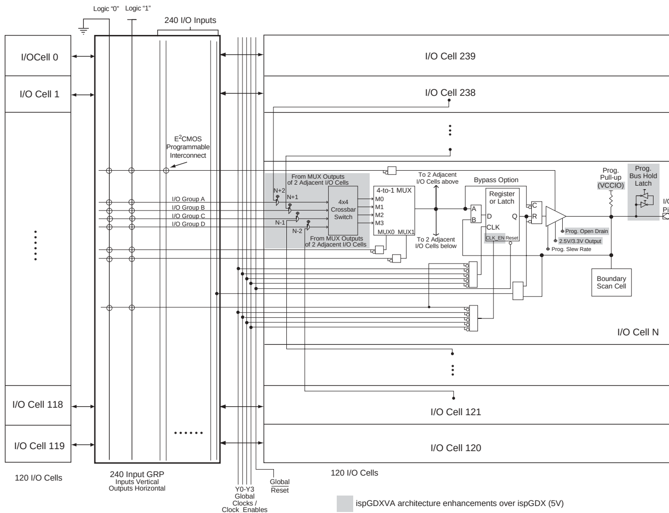
Figure 1. ispGDXVA I/O Cell and GRP Detail (240 I/O Device)
