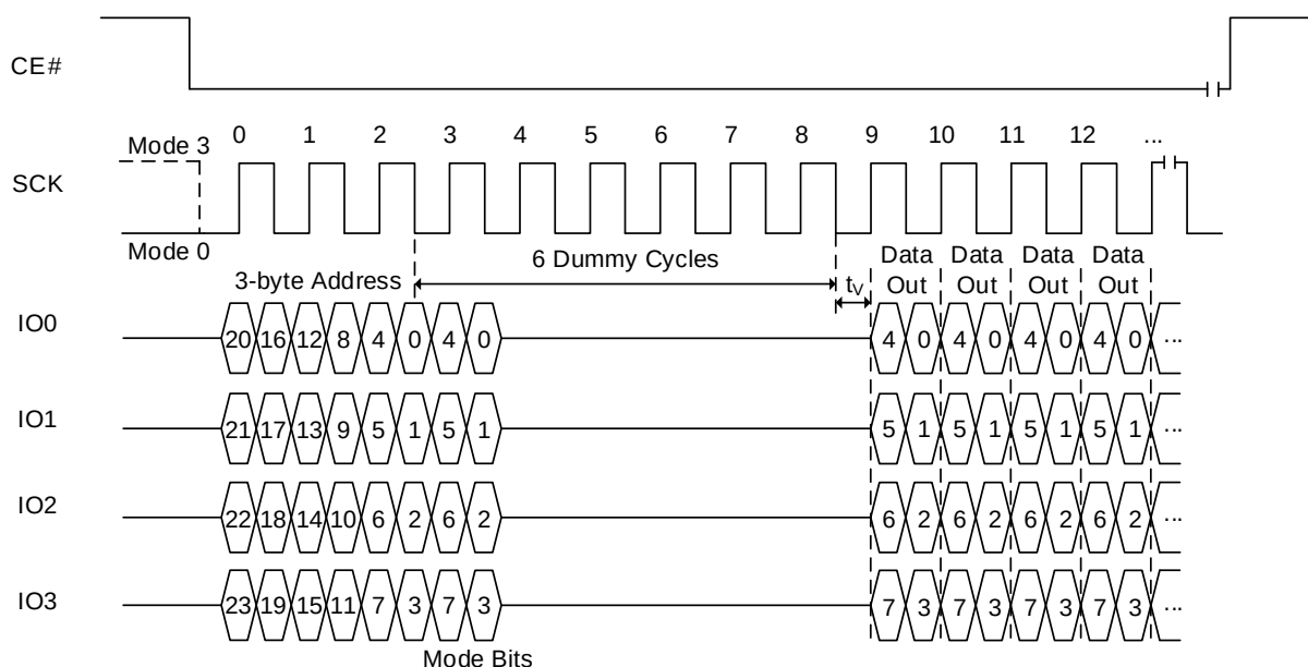
Figure 8.68 FRQDTR Sequence In SPI Mode (without command decode cycles)
