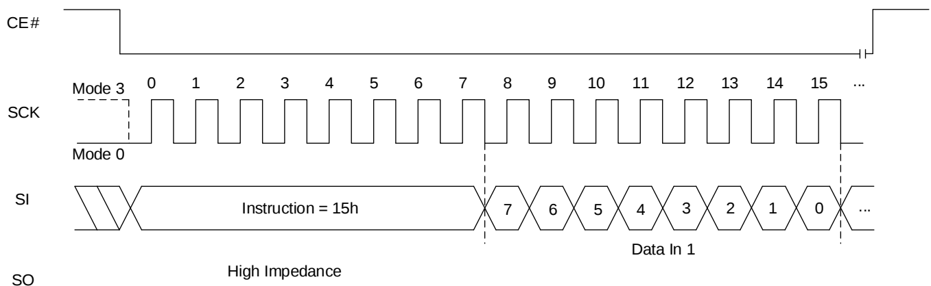
Figure 8.76 WRABR Sequence
