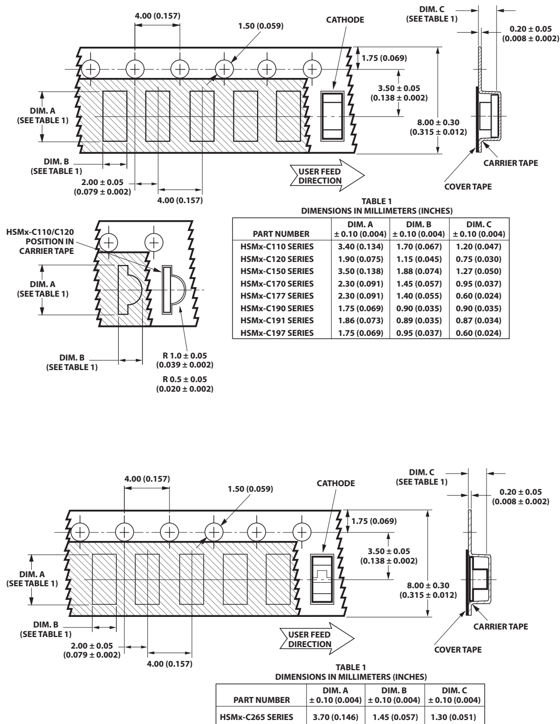
Figure 19. Tape dimensions.
