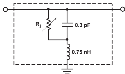
Figure 11. Equivalent Circuit.
