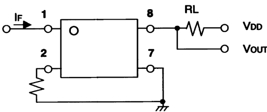
G3VM-352J, -352J(TR)
