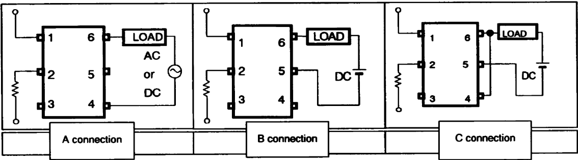
G3VM-351B, -353B
