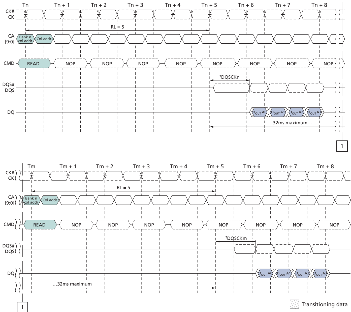
Figure 22: t_{DQSKDL} Timing
