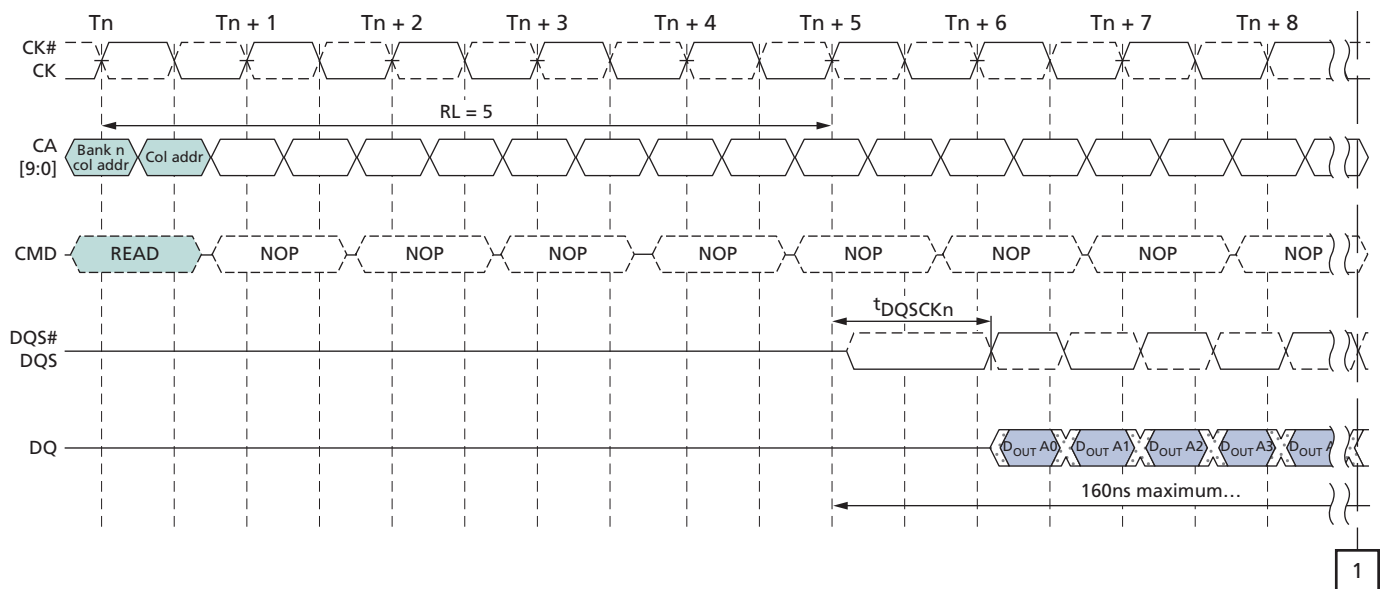
Figure 24: t_{DQSKDS} Timing
