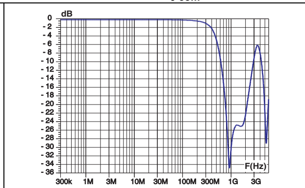
Figure 4. S_{cc21} common mode attenuation measurements ( Z_{0\text{ com}} = 50\ \Omega )
