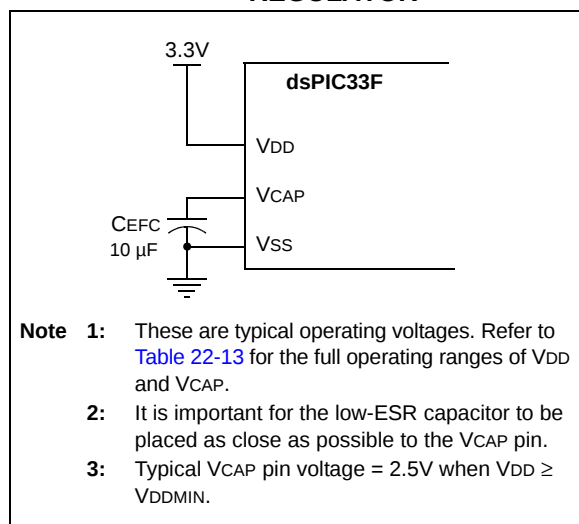
FIGURE 19-1: CONNECTIONS FOR THE ON-CHIP VOLTAGE REGULATOR (1)
