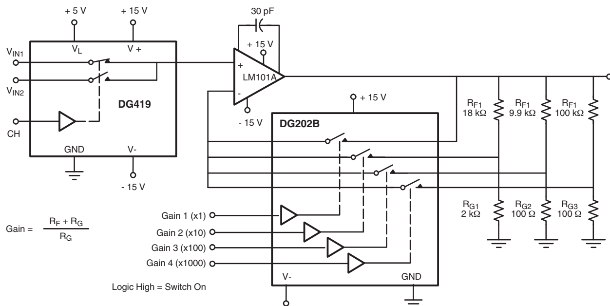
Figure 8. A Precision Amplifier with Digitally Programable Input and Gains
