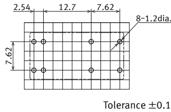
Recommended PC board pattern (BOTTOM VIEW)
