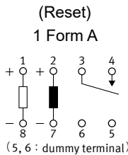
Schematic (BOTTOM VIEW) (Reset)
