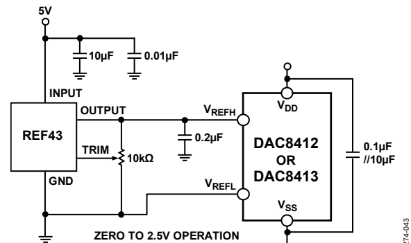
Figure 42. +5\ \text{V} Single-Supply Operation
