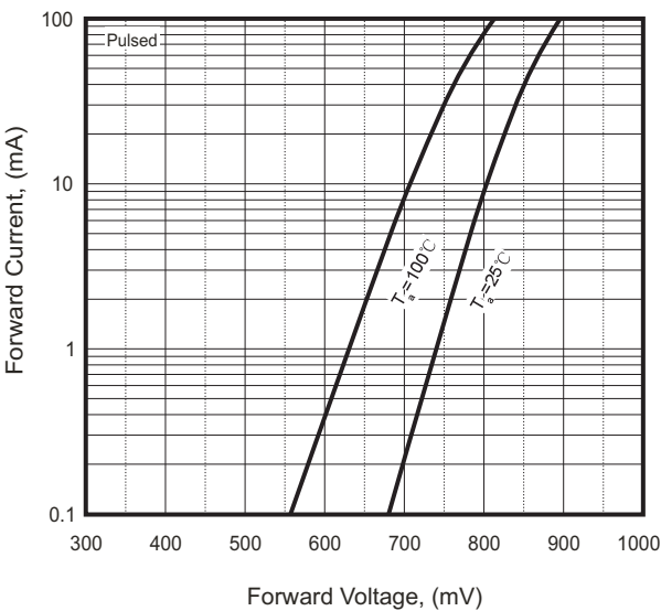
Fig.2 - Forward Characteristics
