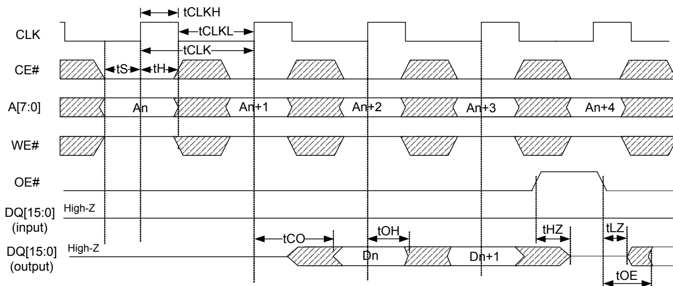
Figure 12. Synchronous Read Timing
