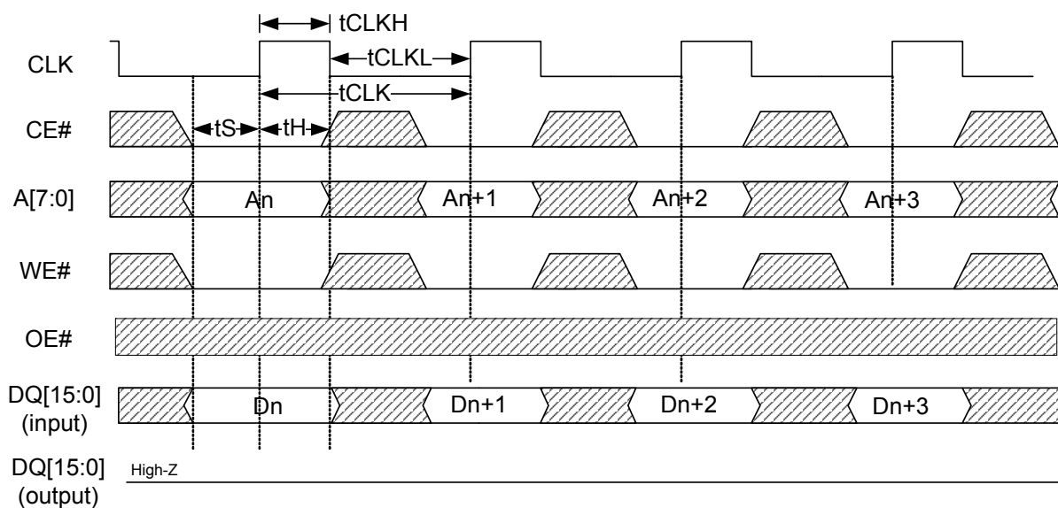
Figure 11. Synchronous Write Timing
