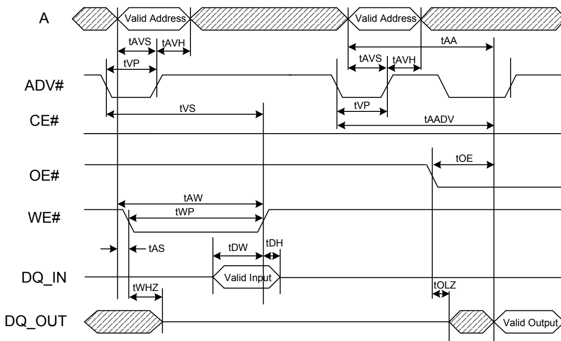
Figure 10. Asynchronous Write to Read Timing
