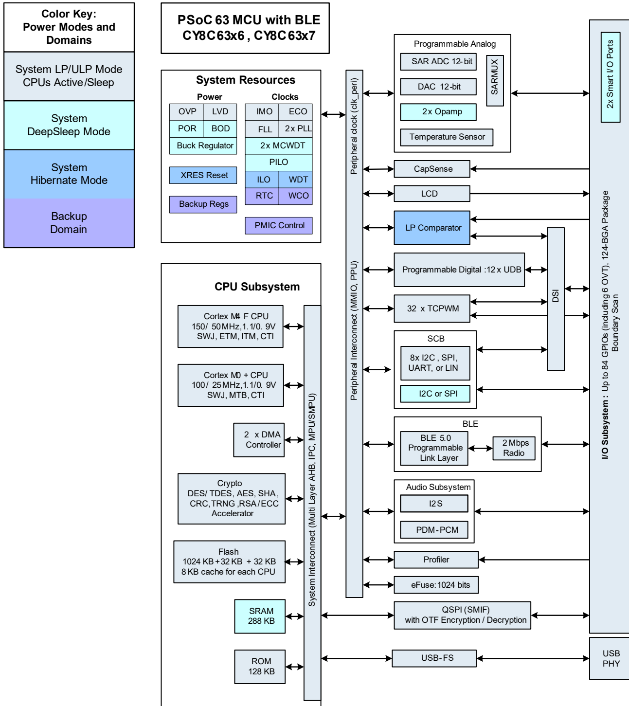
Figure 3. Block Diagram
