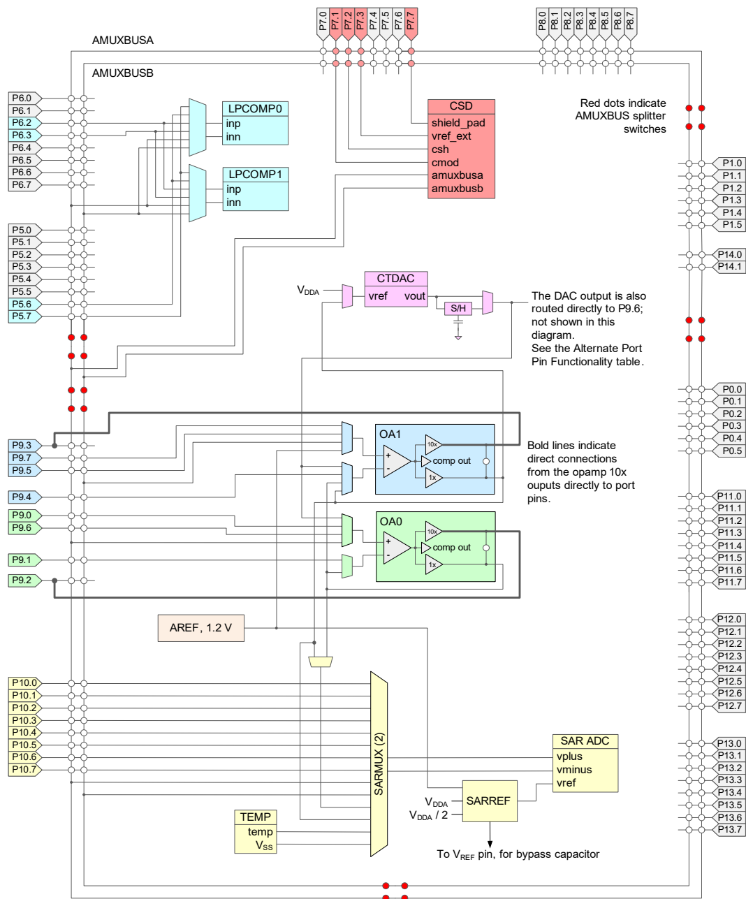
Figure 7. Analog Subsystem
