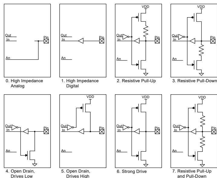
Figure 6-12. Drive Mode
