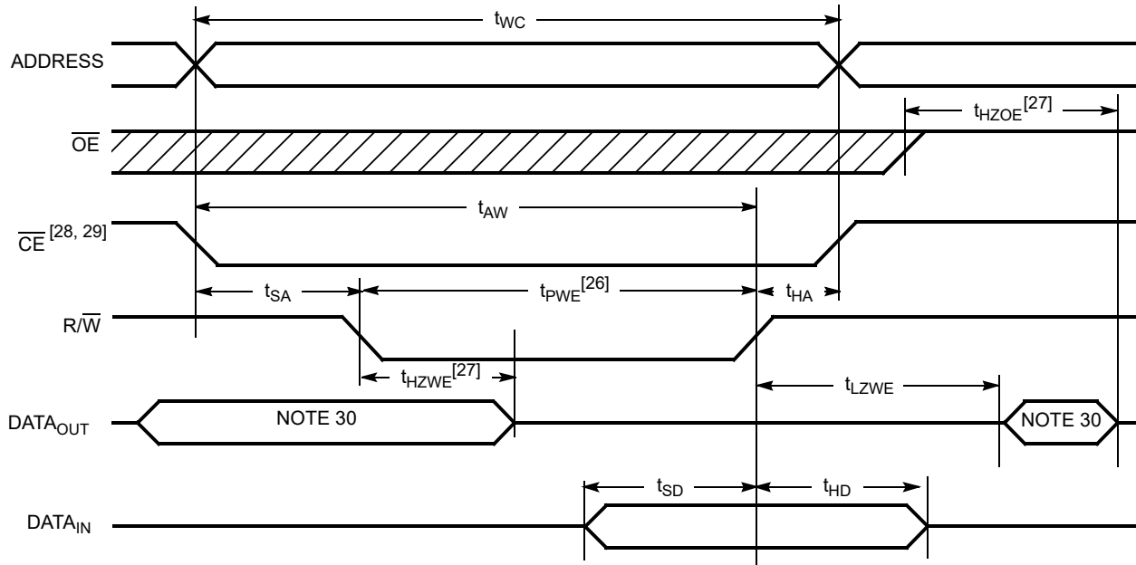
Figure 7. Write Cycle No. 2 ( \overline{CE} Controlled Timing) [23, 24, 25, 31]
