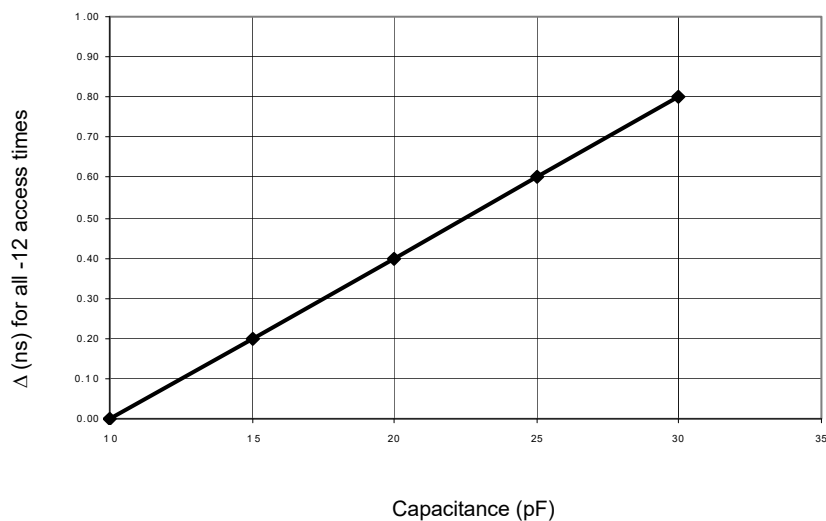
Load Derating Curve
