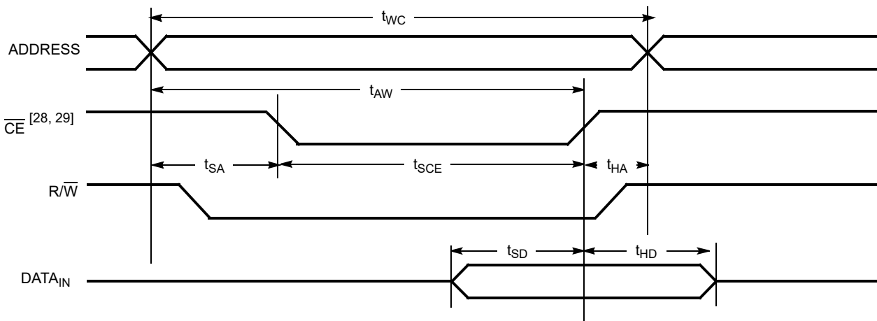
Figure 7. Write Cycle No. 2 ( \overline{CE} Controlled Timing) [23, 24, 25, 31]
