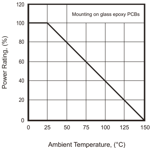
Fig.4 - Power Rating Derating Curve
