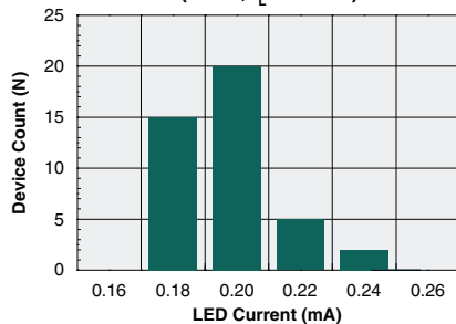
Typical I_F for Switch Dropout (N=50, I_L=600\text{mA} )
