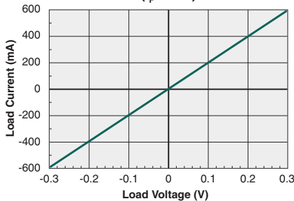
Typical Load Current vs. Load Voltage ( I_F=1\text{mA} )
