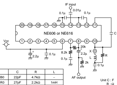
NE(SA)606/616
