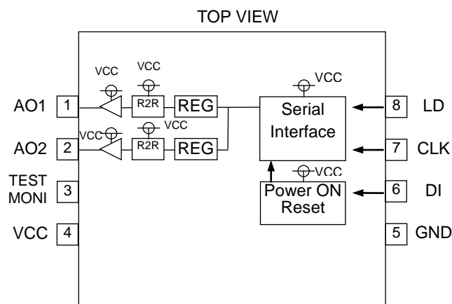
Figure 1. BH2219FVM
