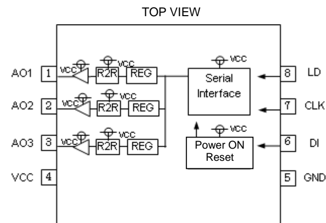
Figure 2. BH2220FVM
