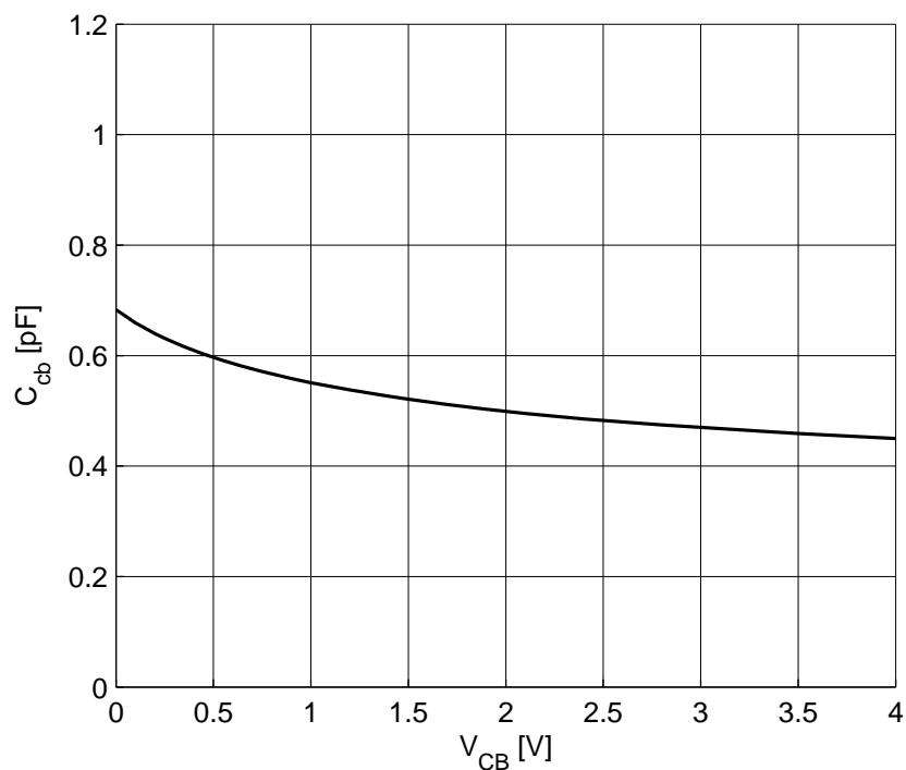
Figure 5-9 Collector Base Capacitance C_{CB} = f(V_{CB}), f = 1 \text{ MHz}
