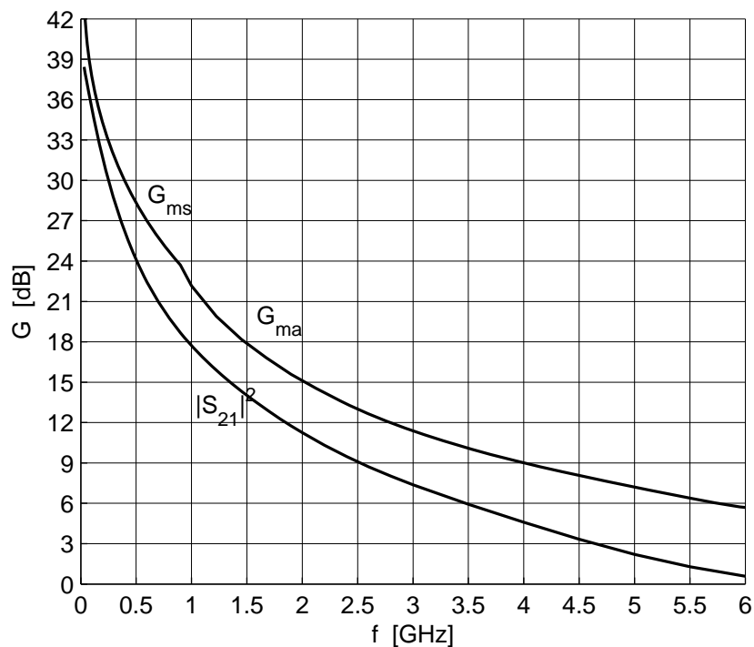
Figure 5-10 Gain G_{ma} , G_{ms} , |S_{21}|^2 = f(f) , V_{CE} = 3 \text{ V} , I_C = 90 \text{ mA}
