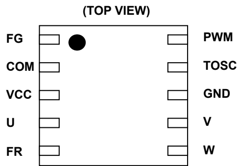
Figure 1. Pin Configuration
