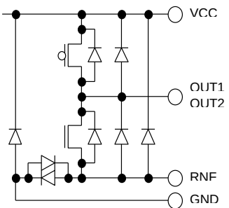
Figure 43. OUT1 / OUT2 (HSOP25)
