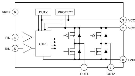
Figure 1. BD6220F / BD6221F
