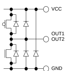
Figure 42. OUT1 / OUT2 (SOP8/HRP7)
