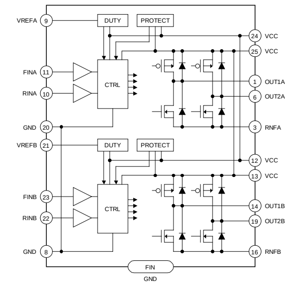
Figure 7. BD6225FP / BD6226FP
