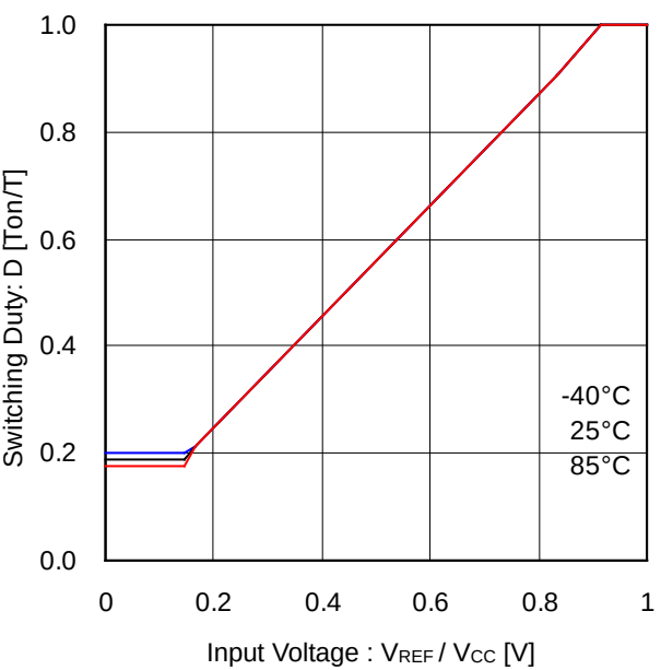
Figure 14. Switching Duty vs Input Voltage (V CC =12V)
