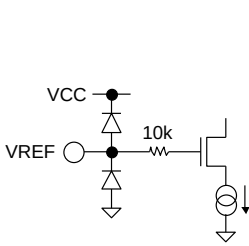
Figure 41. VREF
