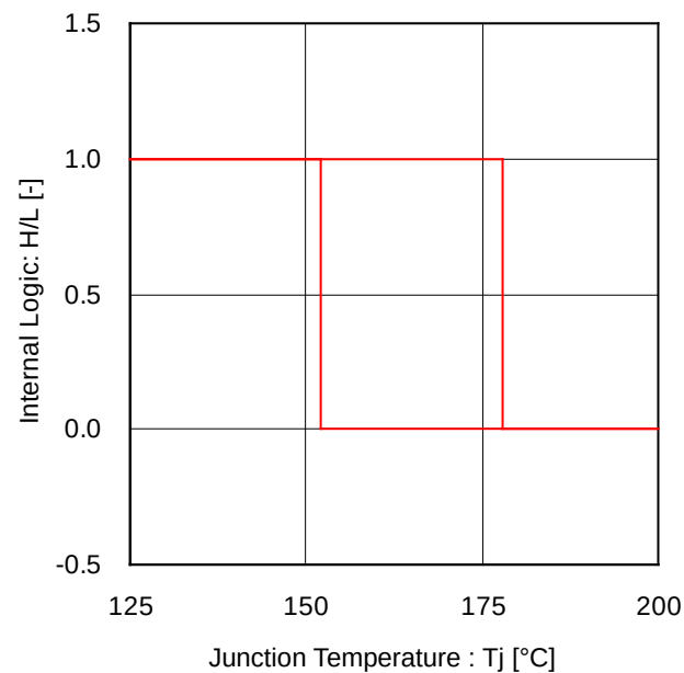
Figure 18. Internal Logic vs Junction Temperature (Thermal Shutdown)
