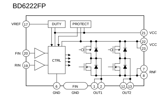
Figure 5. BD6222FP
