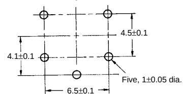
PCB Mounting (Top View) (Single-sided PCB, t=1.6)
