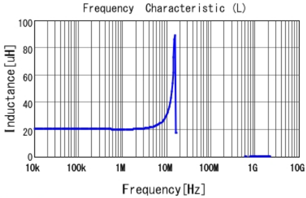
B1047AS-220M L
