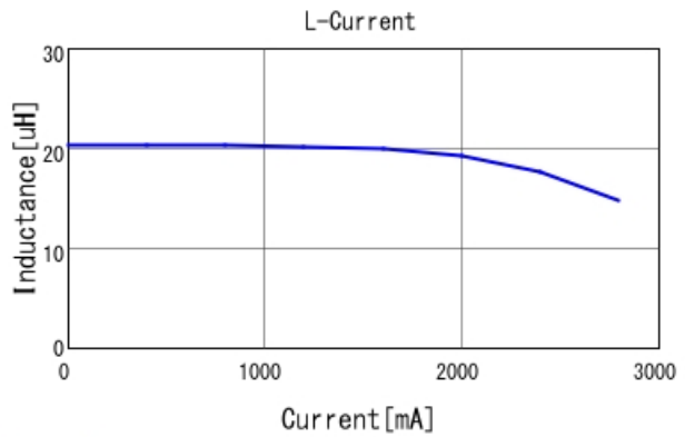
B1047AS-220M L-Current 20degC
