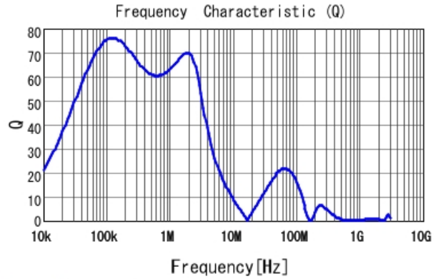
B1047AS-220M Q
