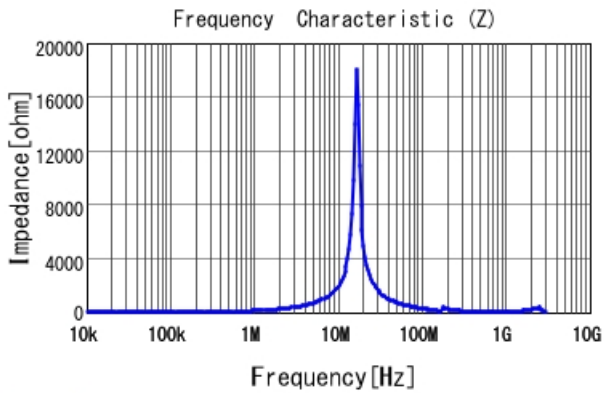
B1047AS-220M |Z|
