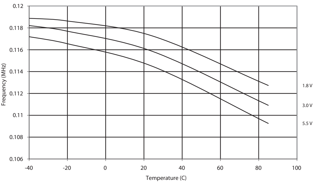
Figure 21-109. Calibrated 8 MHz RC Oscillator Frequency vs. V CC
