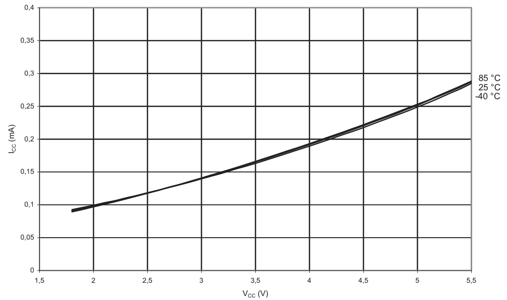
Figure 21-121. Idle Supply Current vs. V_{CC} Internal RC Oscillator, 128 kHz
