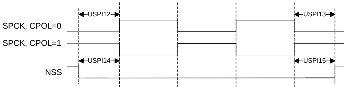
Figure 9-11. USART in SPI Slave Mode, NPCS Timing
