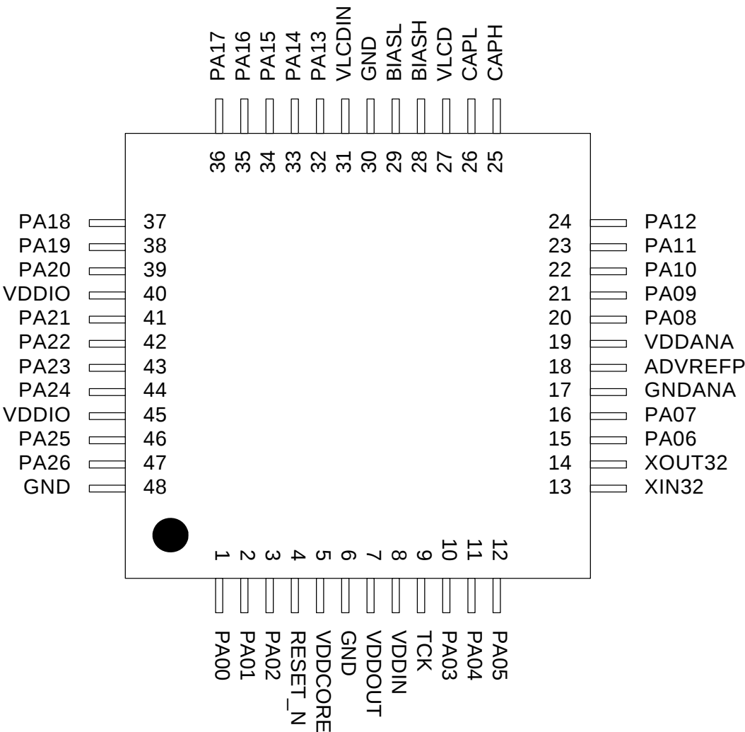
Figure 3-5. ATSAM4LC TQFP48/QFN48 Pinout
