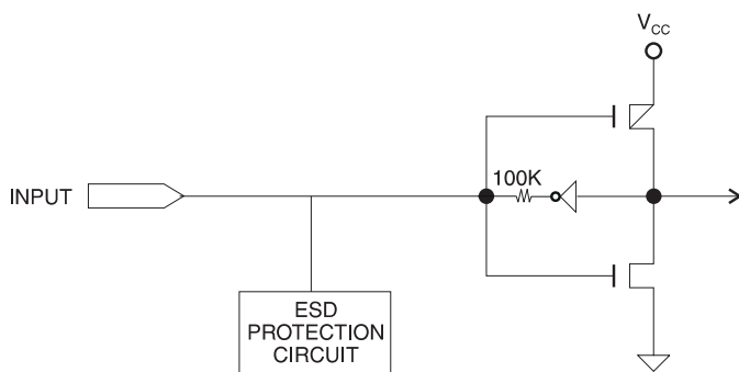
Figure 8-1. Input Diagram
