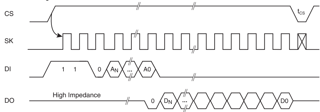
Figure 5-2. READ Timing
