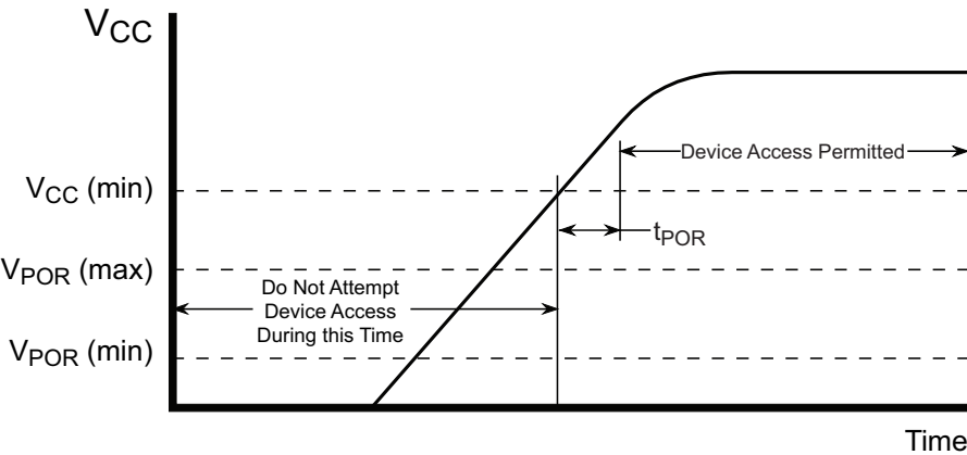
Figure 7-2. Power-Up Timing
