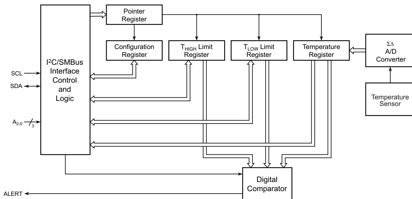
Figure 2-1. Block Diagram
